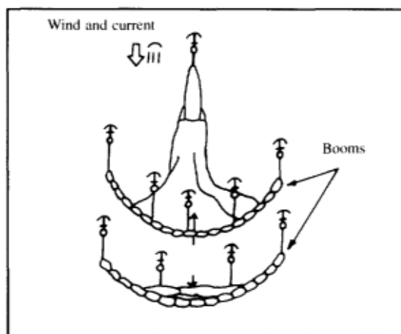
Figure 41: WAYLAYING
