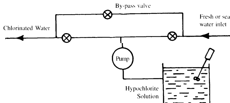
Figure 8 : CHLORINATION TREATMENT
