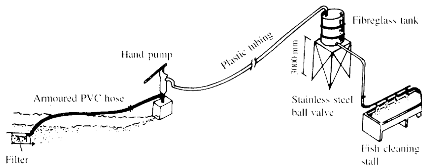
Figure 18 TYPICAL PUMPING ARRANGEMENTS FOR EITHER SEA WATER OR POTABLE WATER
