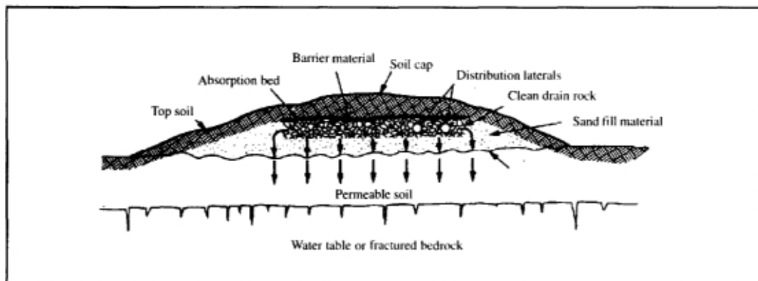
Figure 54b : MOUND SYSTEM
