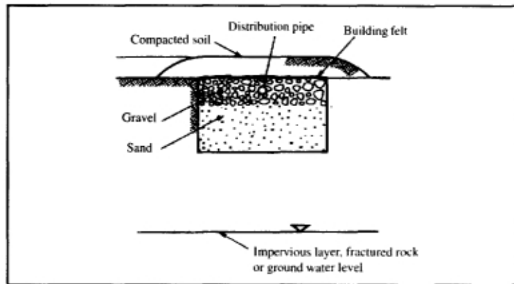
Figure 54a : MIALLUW SAND-FILLED FTELD TRENCH
