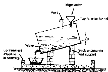
Figure 34a Artisanal oil/water separator
