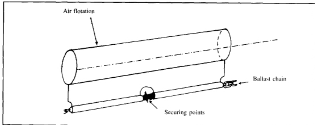
Figure 39 : INFLATABLE BOOM
