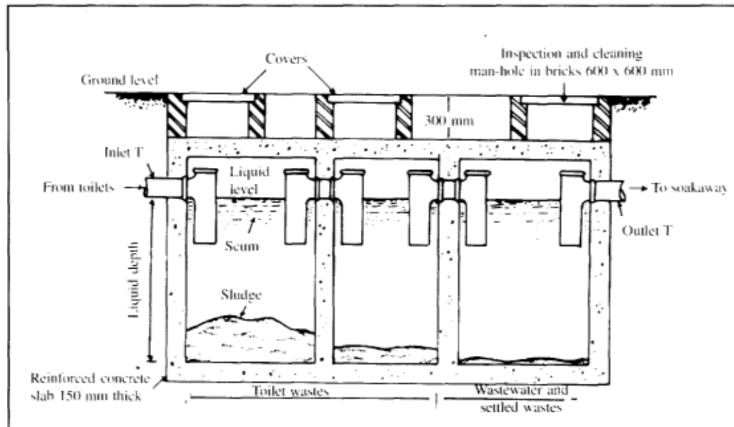
Figure 50 : TRADITIONAL 3-STAGE SEPTIC TANK
