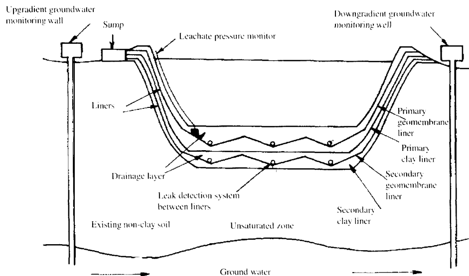
Figure 30 : LANDFILL DOUBLE COMPOSITE LINER
