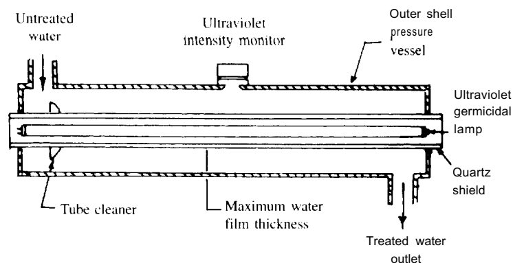
Figure 11 : ULTRAVIOLET IRRADIATION TREATMENT
