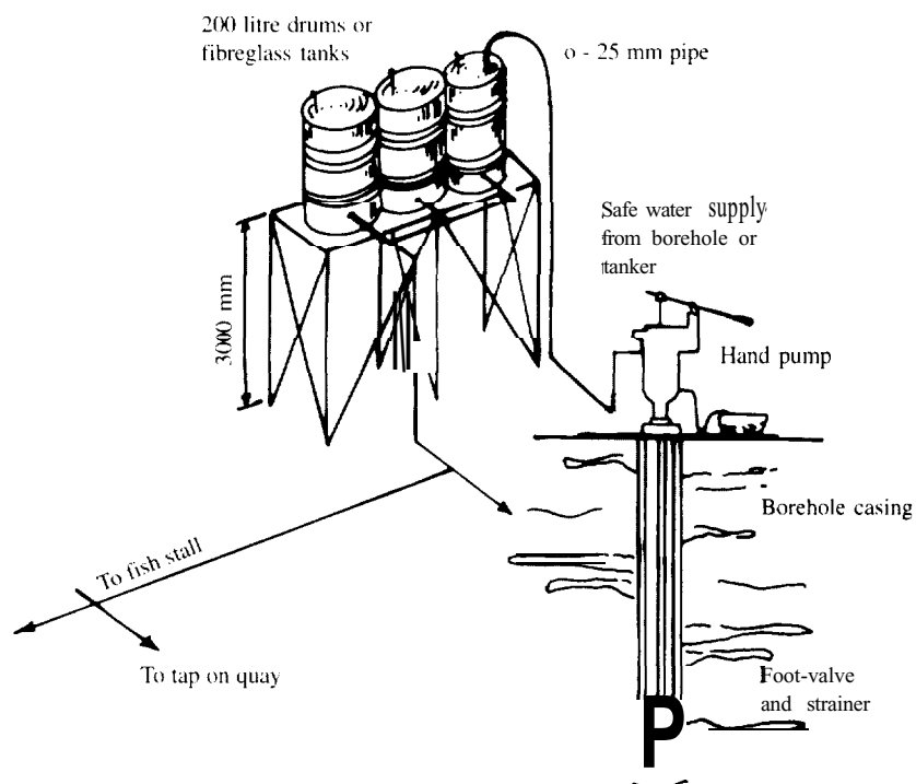
Figure 16 : WATER SUPPLY SCHEME FOR AN ARTISANAL LANDING
