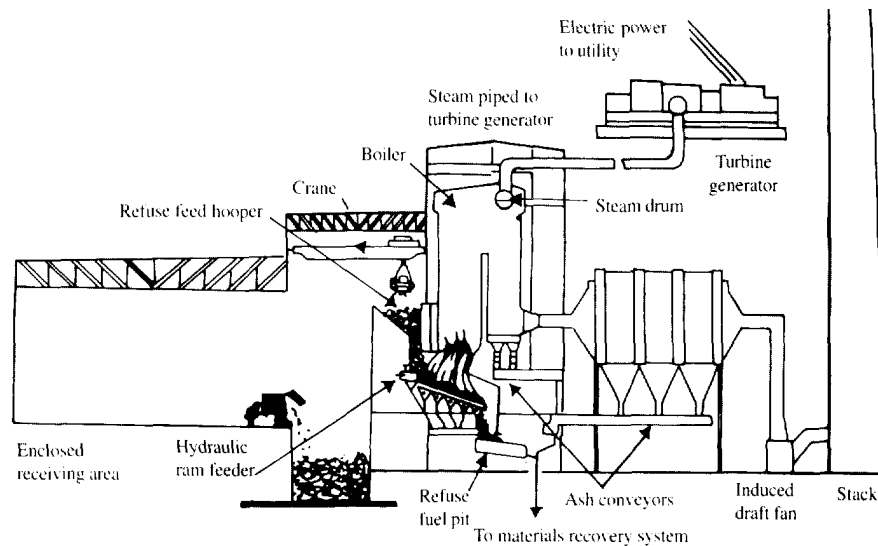
Figure 31 : A TYPICAL CROSS-SECTION OF INCINERATION PLANT
