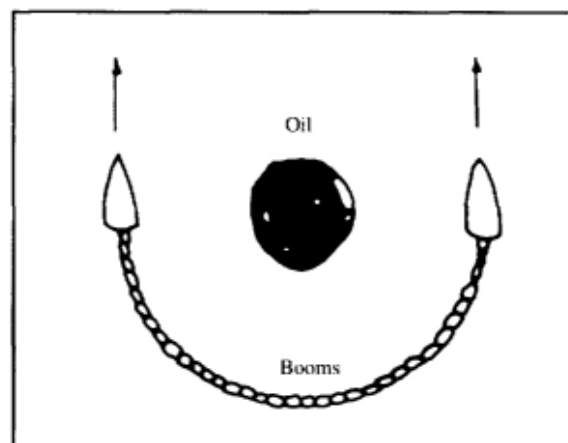
Figure 42 : TOWING
