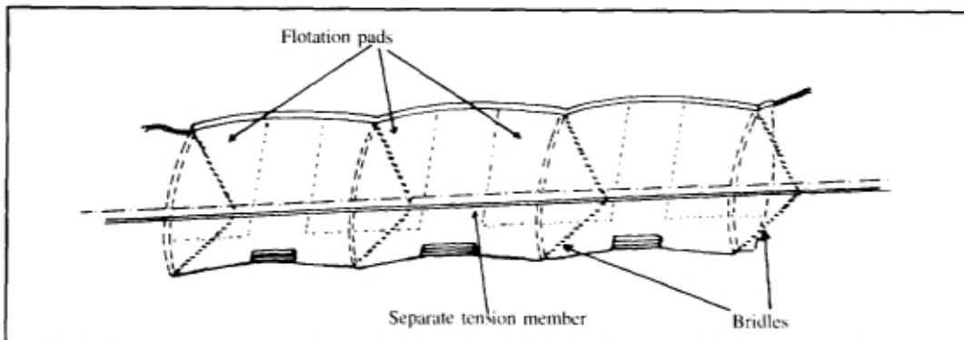
Figure 40 : FENCE BOOM
