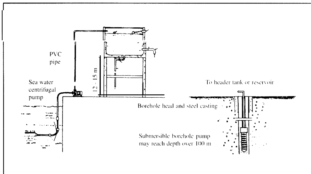
Figure 18 TYPICAL PUMPING ARRANGEMENTS FOR EITHER SEA WATER OR POTABLE WATER
