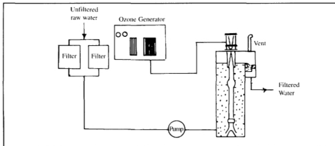
Figure 10 : OZONE TREATMENT
