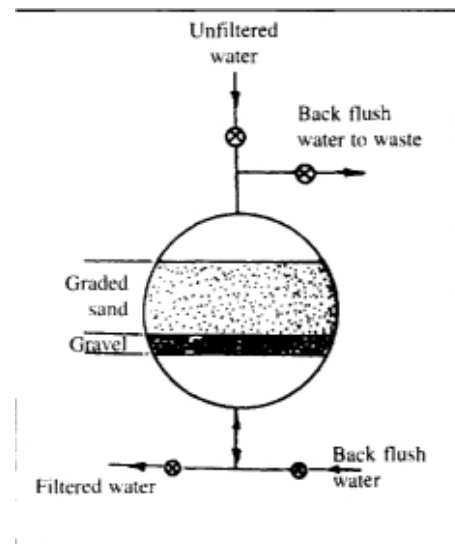
Figure 12 RAPID SAND FILTRATION
