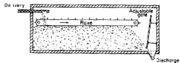
Figure 22c : Ice store with raker
