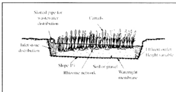
Figure 52b: : SUBSURFACE WATER FLOW TREATMENT
