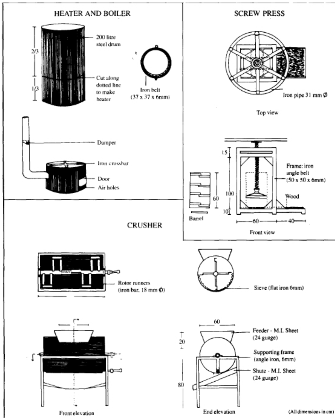
Figure 60: COMPONENTS OF A MINI FISH MEAL PLANT
