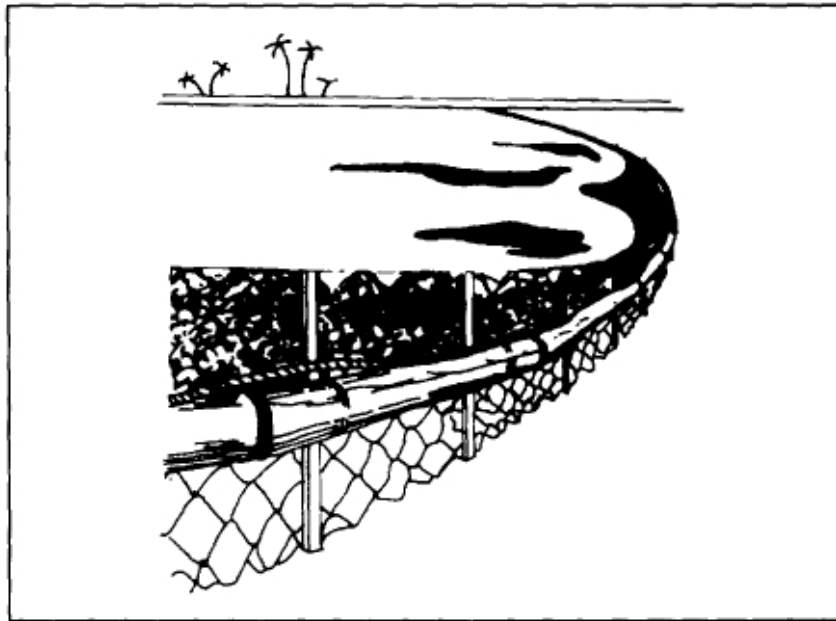
Figure 38 : An artisanal floating oil boom made from bamboo floaters, pieces of timber uprights and fish net fillet with rice straw sorbent. The sorbent can be dried and incinerated ashore.
