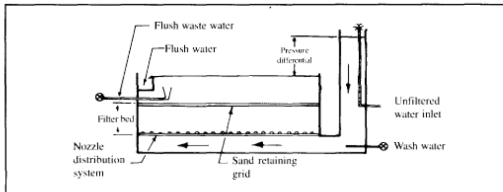
Figure 15a : ATMOSPHERIC PRESSURE UP-FLOW FILTER
