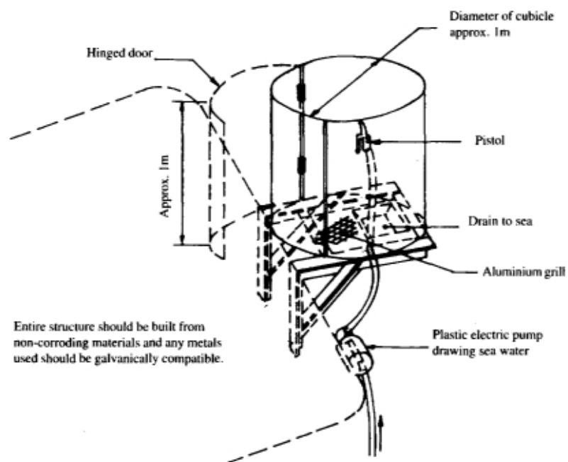
Figure 68: A WALK-IN FACILITY
