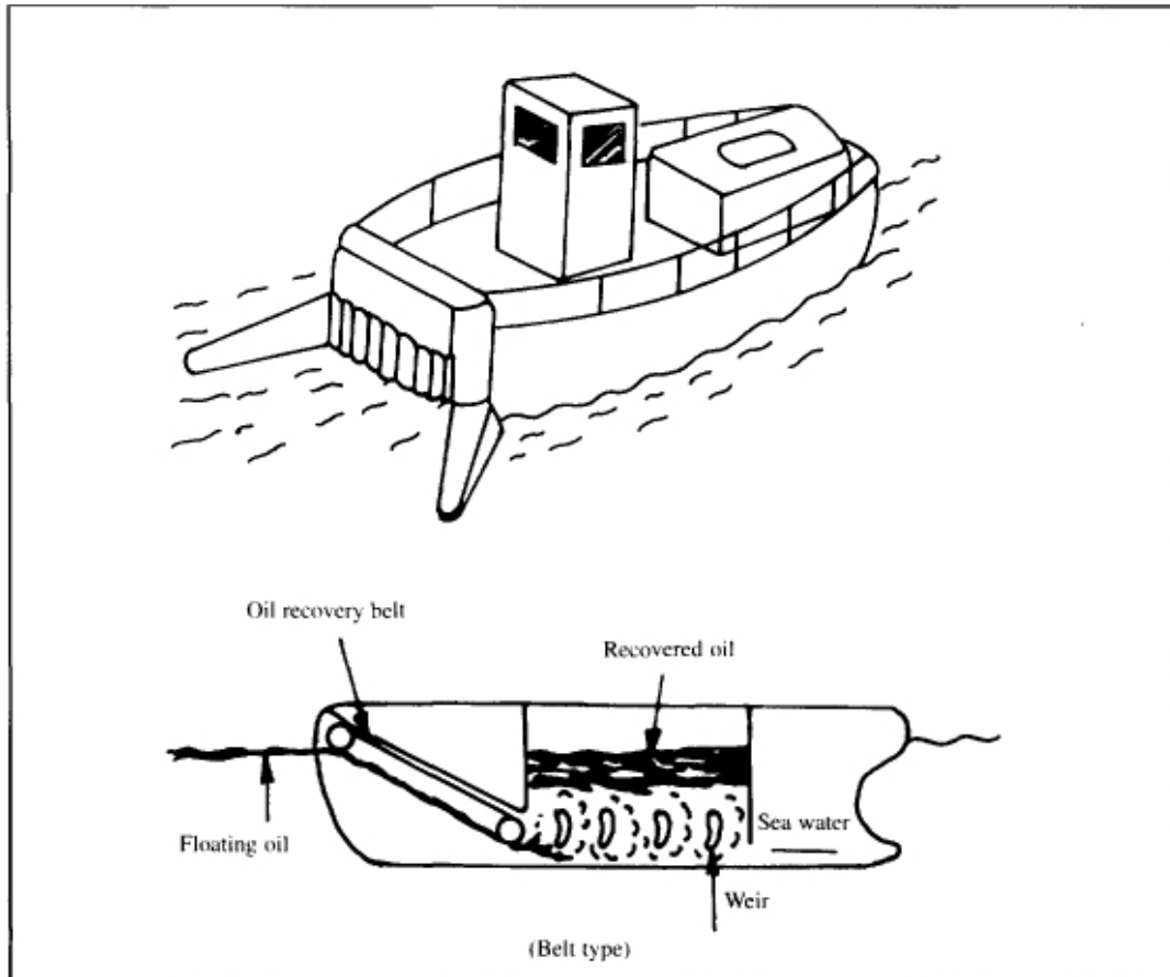
Figure 46: INDUCTION TYPE OIL SKIMMER
