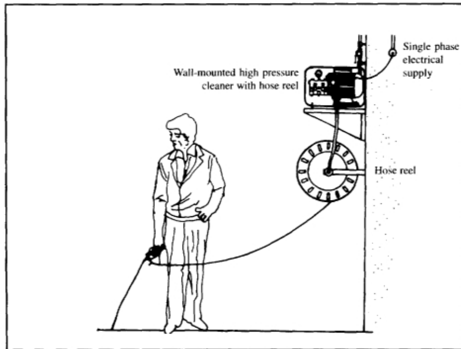
Figure 57b . Shows a fixed high pressure cleaner mounted on the wall. Small units like this are also very suitable for cleaning fish baskets, which generally require copious amounts of running water
